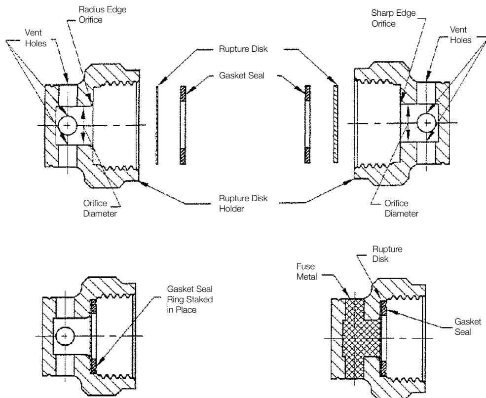
PRESSURE RELIEF DEVICE SELECTION CHART
