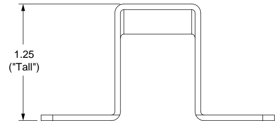
00CMK-0032-00 Cylinder Mounting Bracket, Tall SCALE 1 : 1
